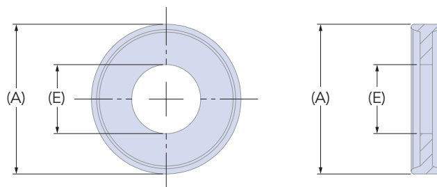
Gasket configurations for all 25.0mm flange sizes
