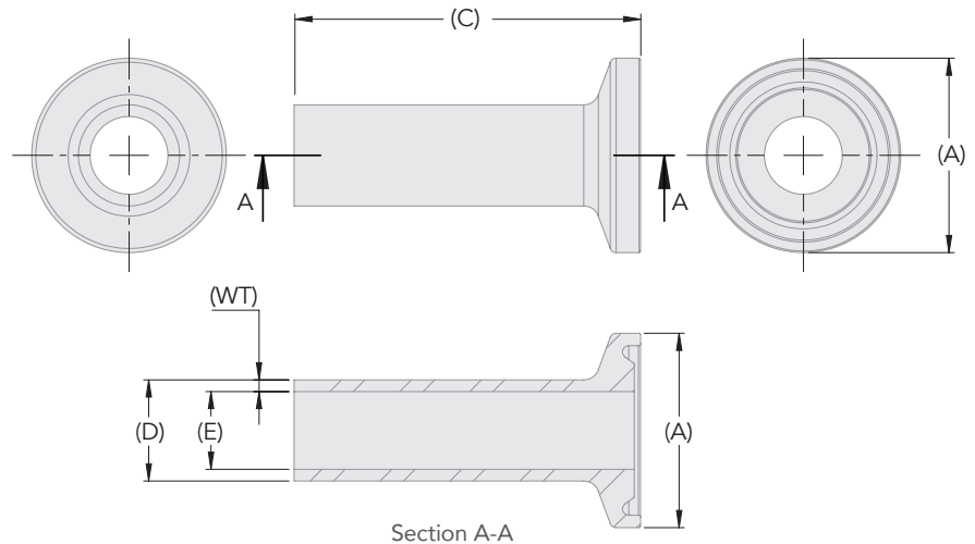
Type A – 25.0mm Flange
