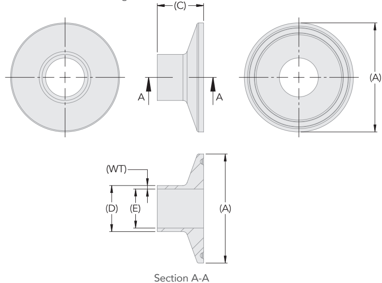
Type B – 34.0mm to 338.0mm Flange
