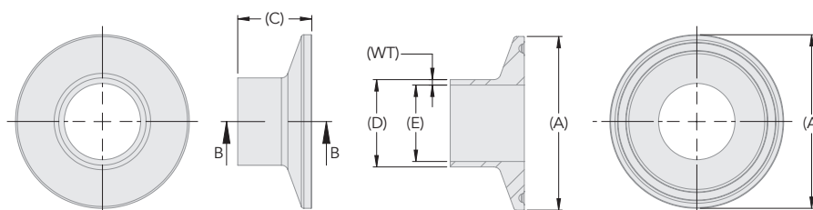
Section B-B
